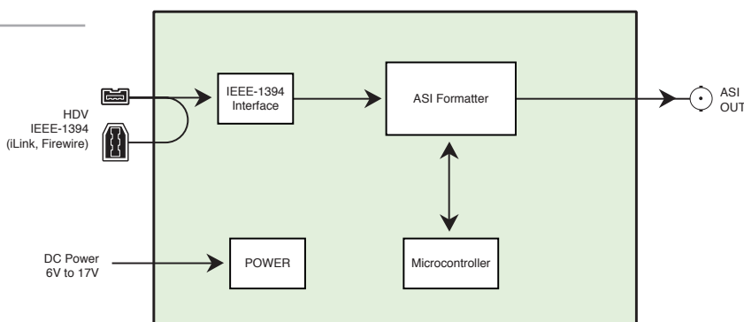
ASI-Bridge Functional Block Diagram
